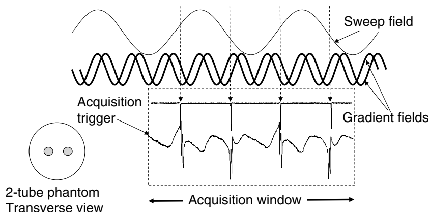
Fig. 4. Direct detected rapid scan absorption EPR signals of a phantom sample consisting of two capillary tubes containing a mg each of particulate TCNQ ( N -methylpyridinium tetracyanoquinodimethane, a stable charge-transfer complex that give an exchange-narrowed single line EPR spectrum) sample. The top sinusoid represents the rapid scan sweep, and the two higher frequency sinusoids represent the X and Z gradients, which together provide the rotating gradient in the XZ plane. The left side of the dotted rectangle represents the start of the trigger. The field scan frequency was 333.33 Hz and the gradient rotation frequency was 1 kHz. The sampling frequency was 4 Ms/s and 25,000 points were collected, giving rise to two downfield scans (first and the third spectrum) and two up field scans (second and the fourth spectrum). The zero-gradient spectra (upper) and the spectra under rotating gradient (lower) at an arbitrary starting phase are shown.
