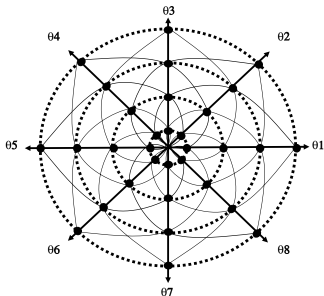
Fig. 2. Mnemonic representation of the way we collect the elements of the B\theta matrix for various CW imaging modalities. The diagonal double-headed arrows (1–5, 2–6, 3–7, 4–8, 5–1, 6–2, 7–3, 8–4) represent conventional projection data collection, with 8 sweeps (B1–B8) each with constant gradient orientation from \theta_1 to \theta_8 . The concentric dotted circles represent the stepped-field-rotating-gradient modality (Ohno et al. [25] and Deng et al. Ref. [12]), and the Kaleidoscopic pattern (continuous lines) represent the simultaneous rapid scan and rotating gradient strategy.
