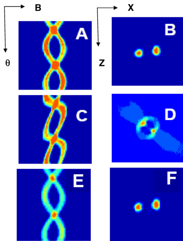
Fig. 6. (A) 2D projections (shown as a sinogram) obtained by rotating the gradient in the XZ plane for 2-tube phantom with the axis perpendicular to the XZ axis and (B) the image of such a phantom via filtered back-projection. (C) 2D pseudo-projections and the corresponding back-projected pseudo-image obtained by transforming the projection matrix that correspond to data that would be obtained by a forward scan of field combined with rotating gradient of the same magnitude as in A and B. (D) The pseudo-image obtained by simply back-projecting the data in C and is not the true image, as expected. (E) Correct sinogram obtained by reshuffling the matrix corresponding to (C). (F) Image obtained by back-projection of (E) which is identical to (B).
